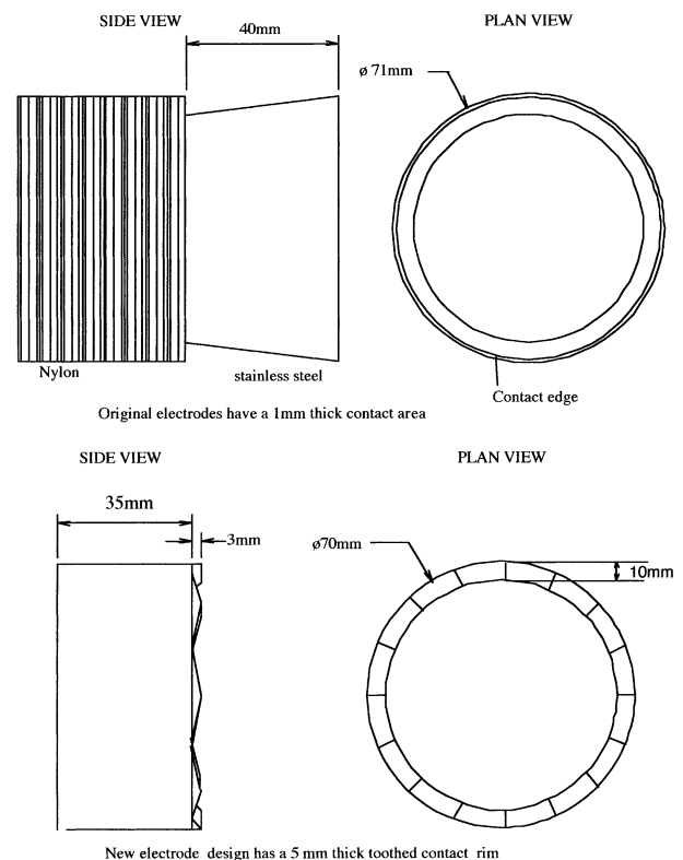
Fig. 1. Original electrodes and suggested improvements.
